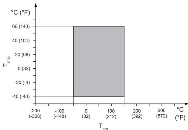
Fig. 18: Allowed process fluid and ambient temperatures, integral type
