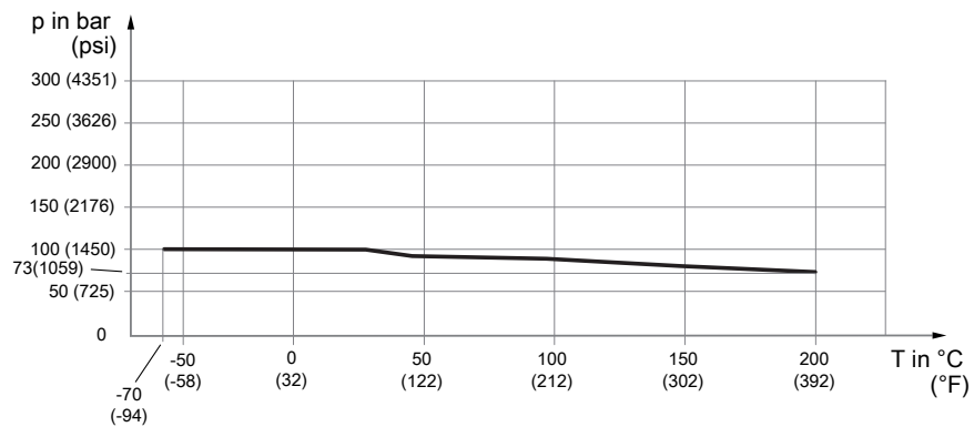
Fig. 17: Allowed process pressure as a function of process connection temperature
