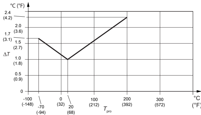
Fig. 10: Temperature accuracy
