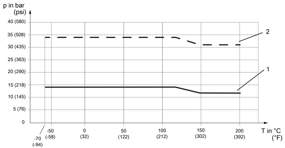
Fig. 16: Allowed process pressure as a function of process connection temperature
