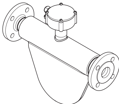
Fig. 20: Remote type sensor with standard neck
