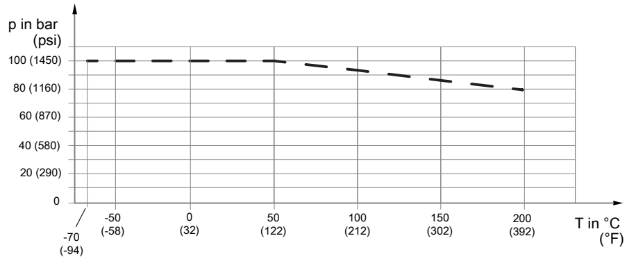
Fig. 15: Allowed process pressure as a function of process connection temperature, suitable for flange EN 1092-1 PN100
