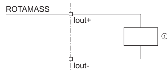
Fig. 24: Active current output connection I out HART
