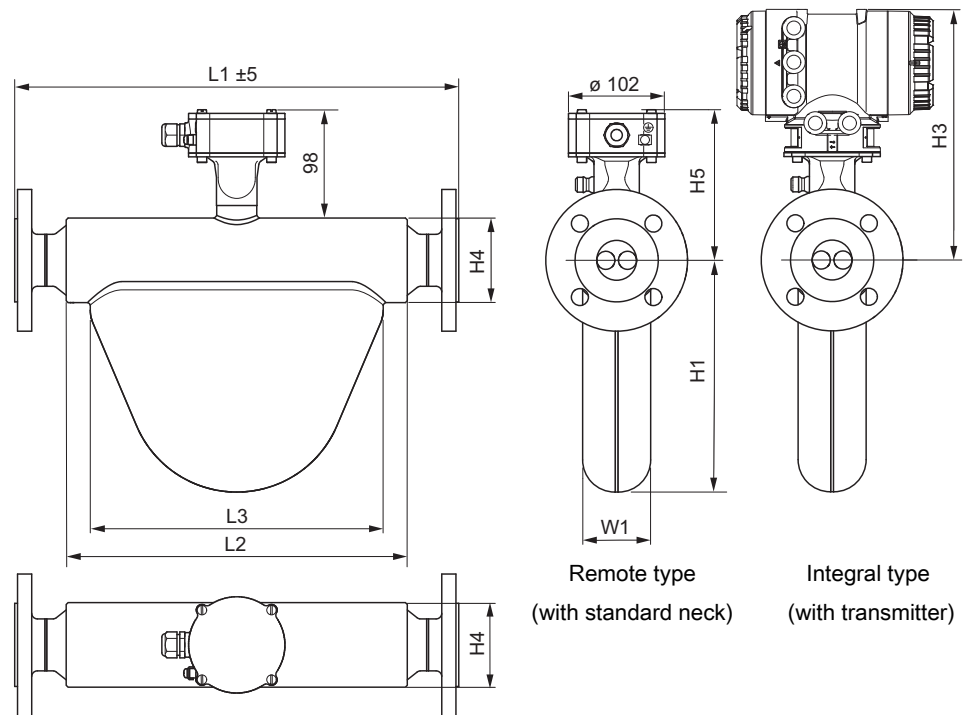
Fig. 21: Dimensions in mm
